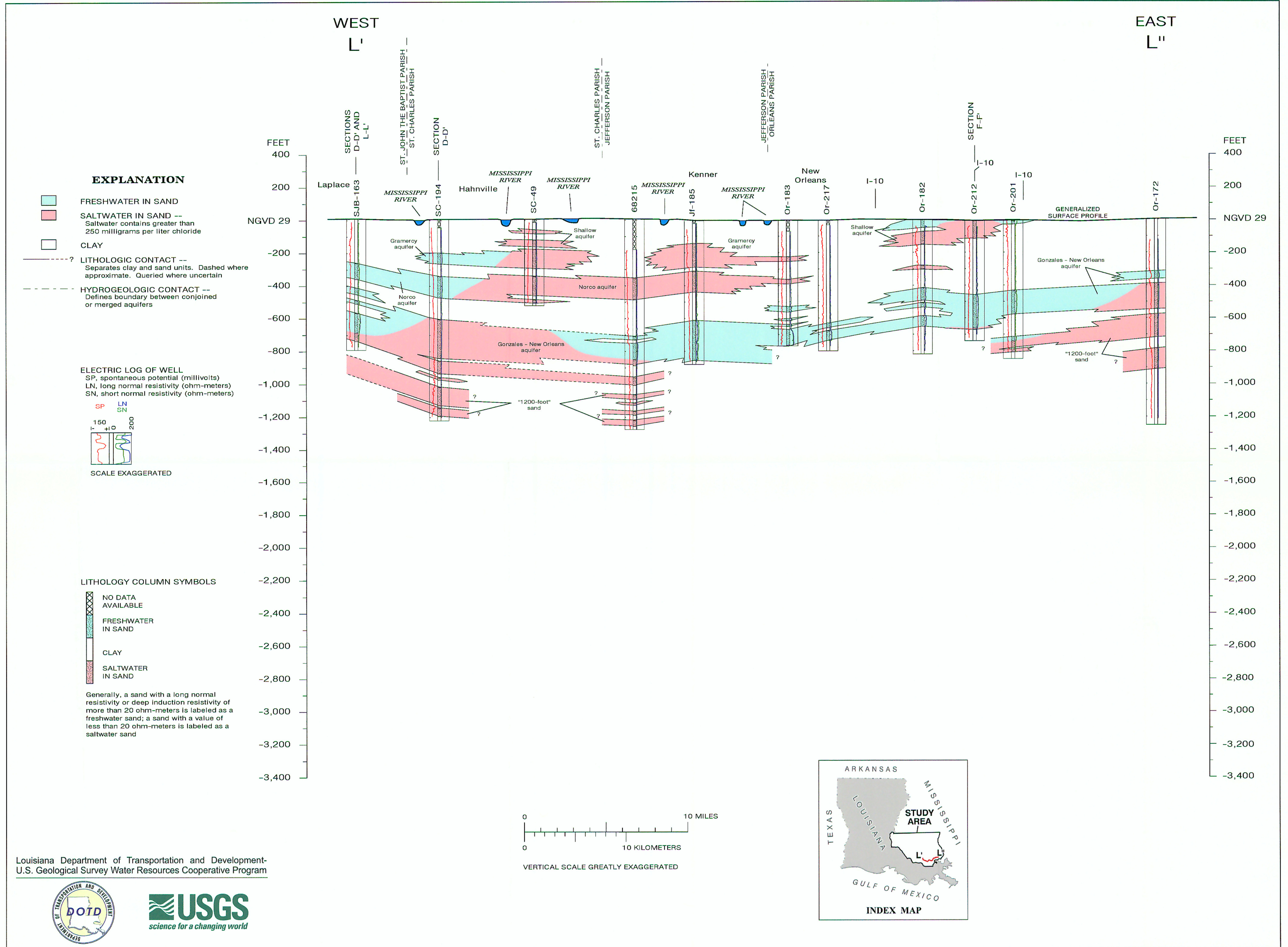
Plate 18. West-to-east hydrogeologic section L'-L'', southeastern Louisiana.
