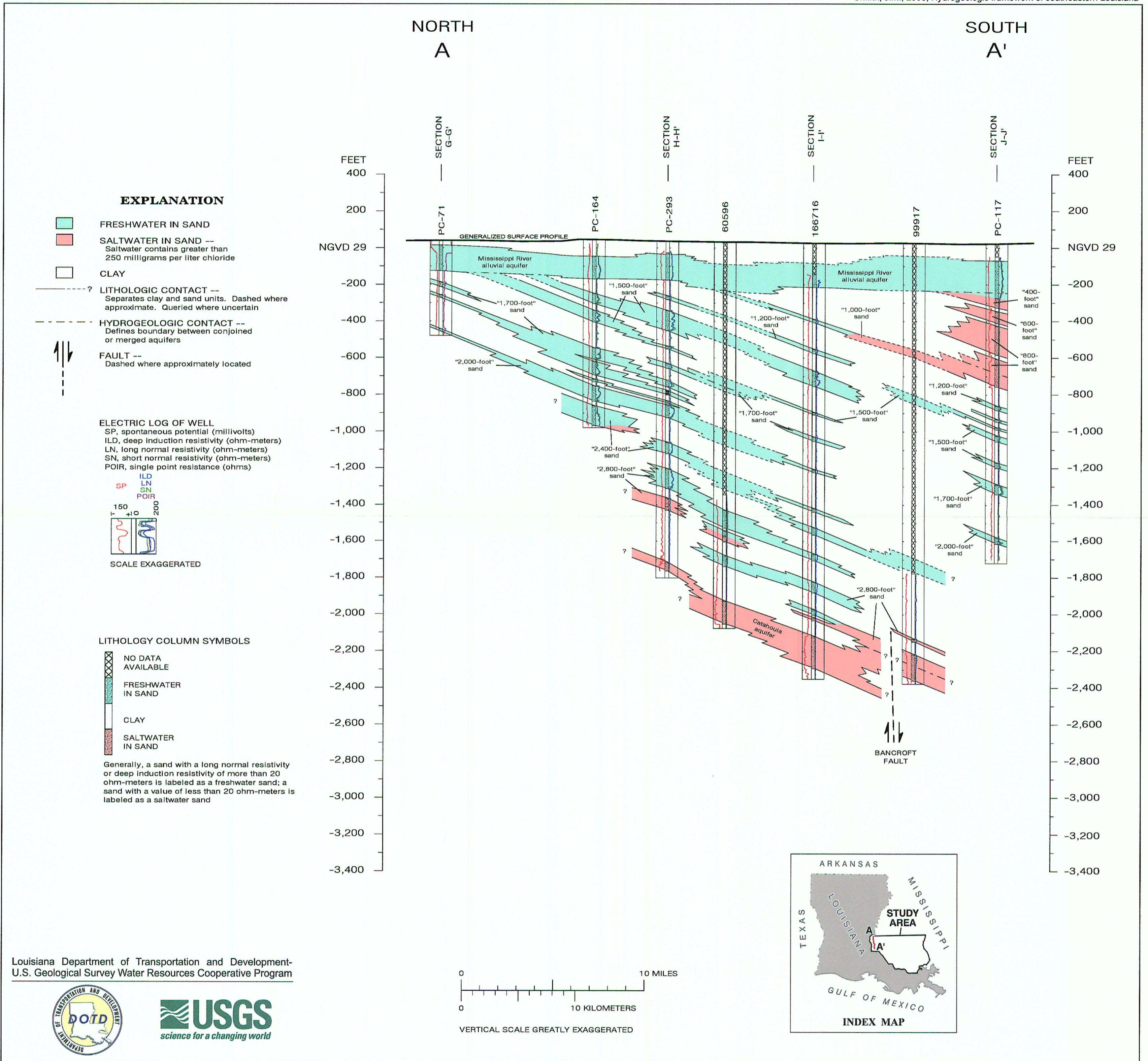
Plate 2. North-to-south hydrogeologic section A-A', southeastern Louisiana.
