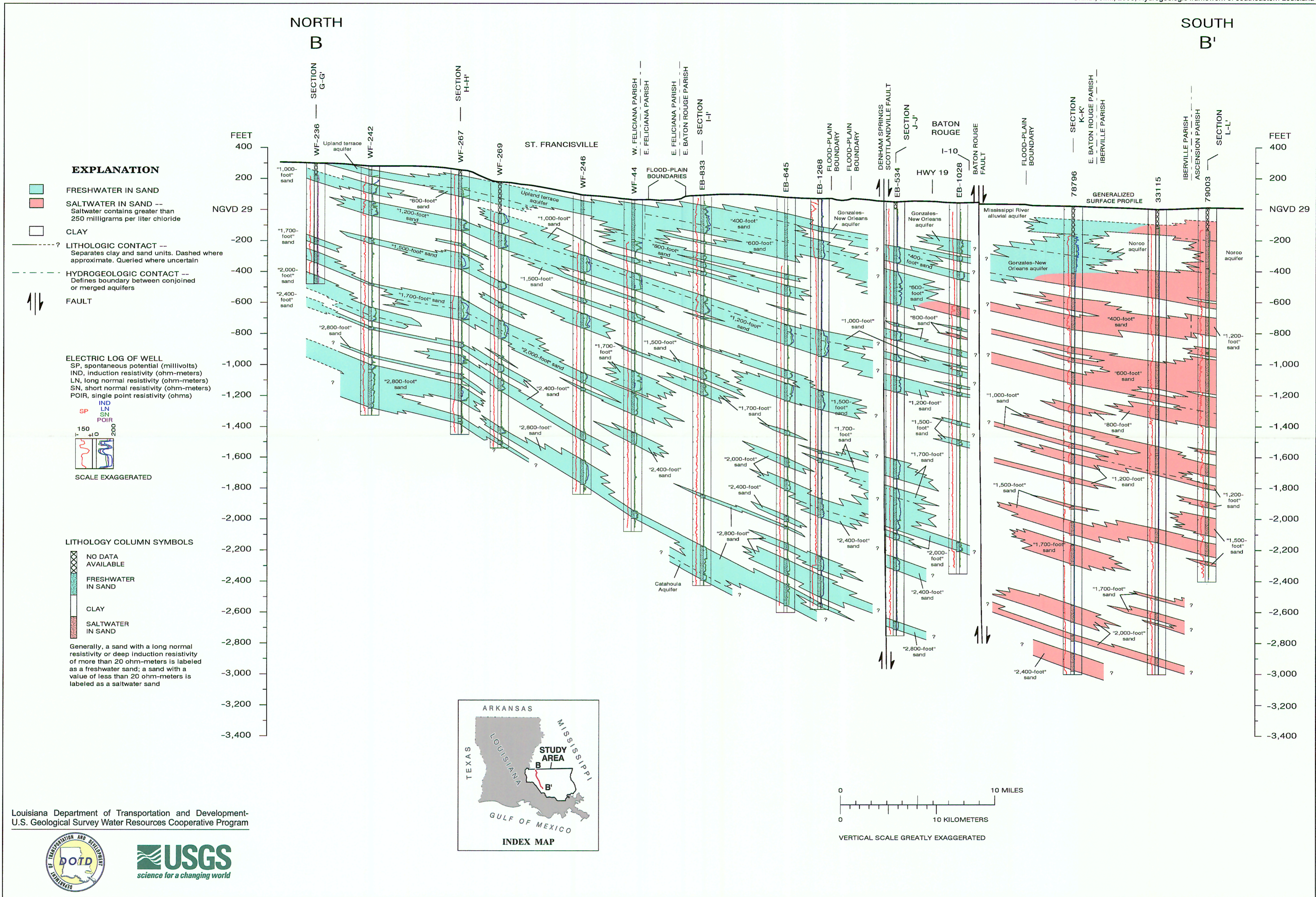
Plate 3. North-to-south hydrogeologic section B-B', southeastern Louisiana.
