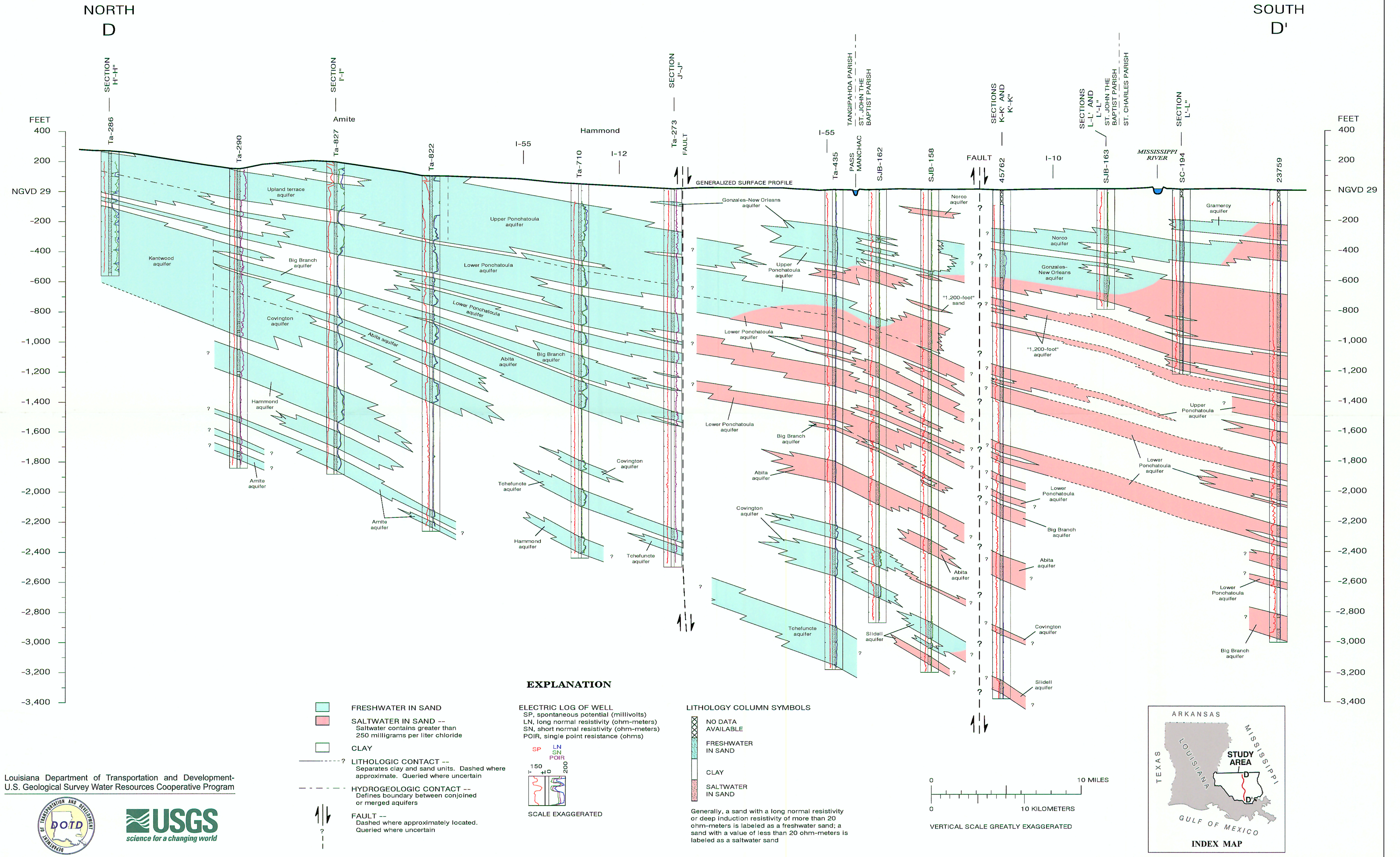
Plate 5. North-to-south hydrogeologic section D-D', southeastern Louisiana (after Nyman and Fayard, 1978, pl. 1).
