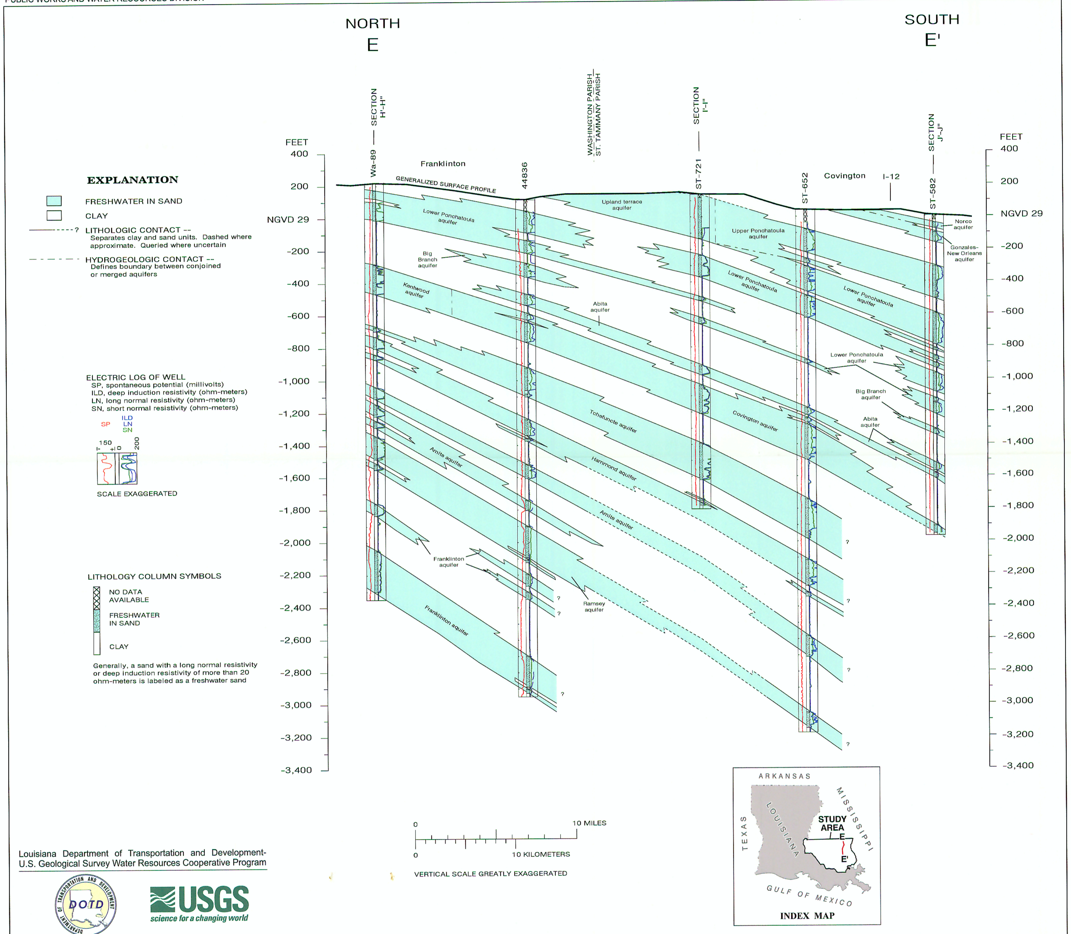
Plate 6. North-to-south hydrogeologic section E-E', southeastern Louisiana.
