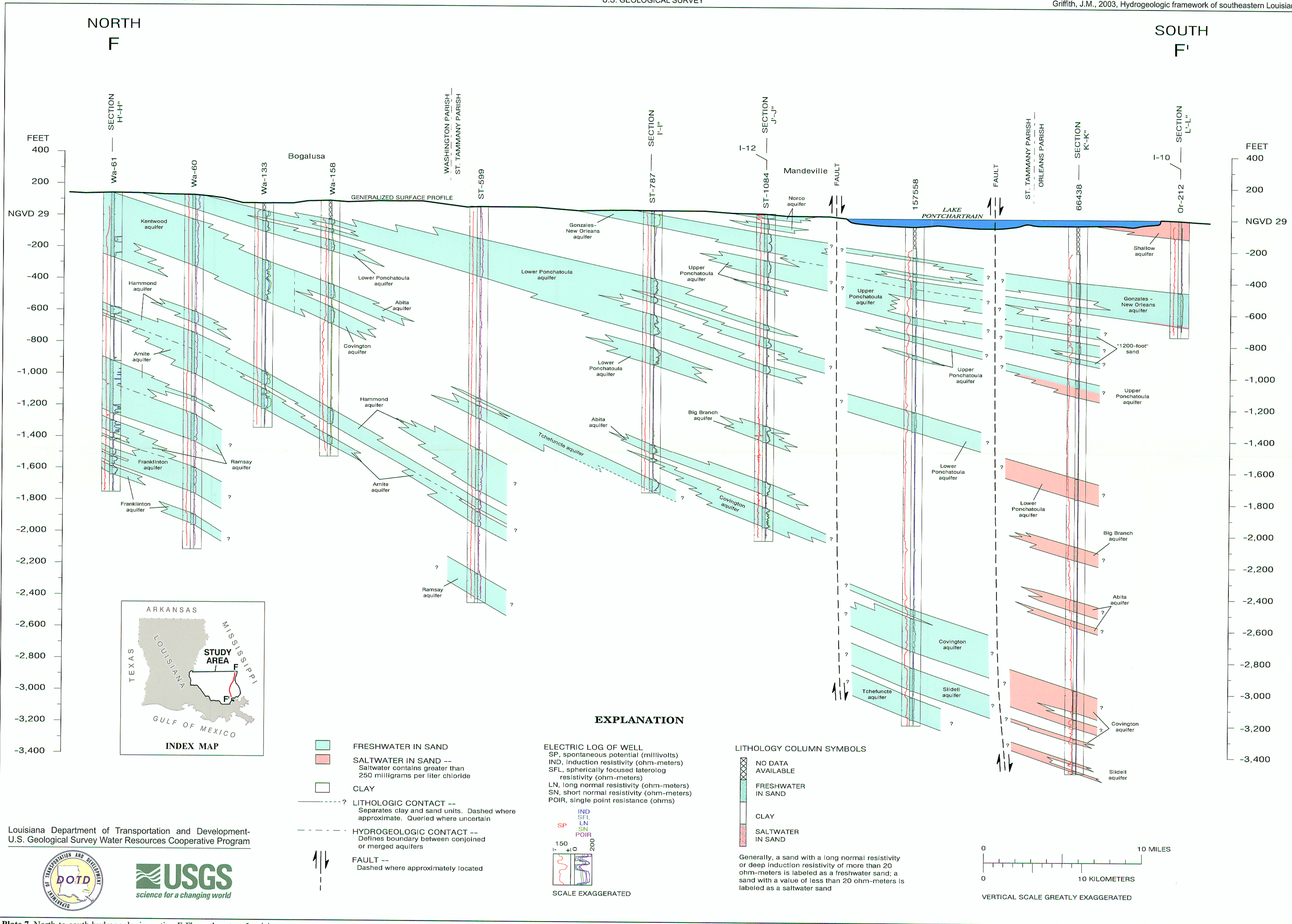
Plate 7. North-to-south hydrogeologic section F-F', southeastern Louisiana.
