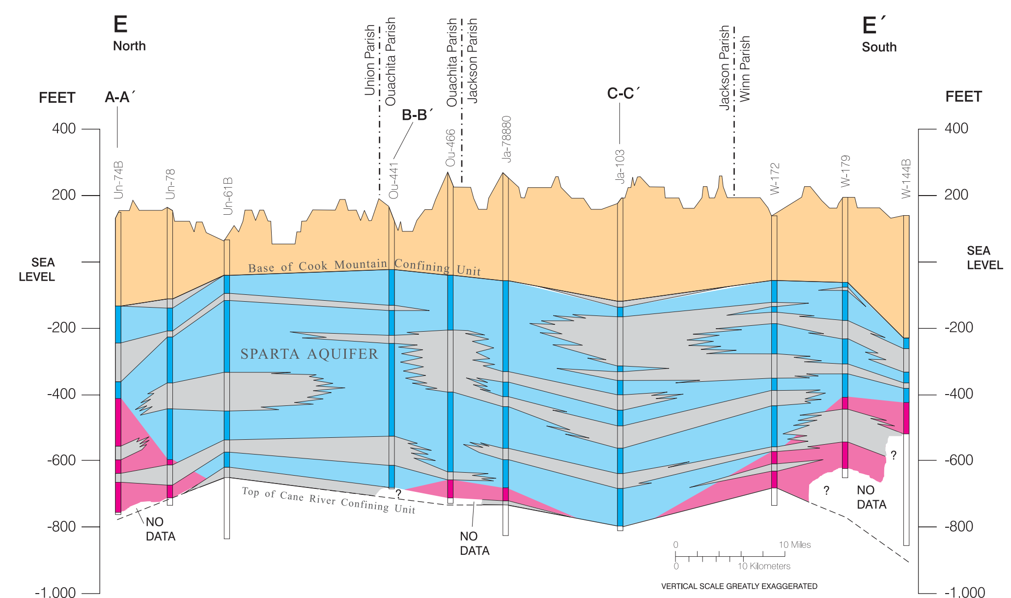
Figure 8. North-to-south hydrogeologic section (E-E') through the Sparta aquifer in northern Louisiana.
