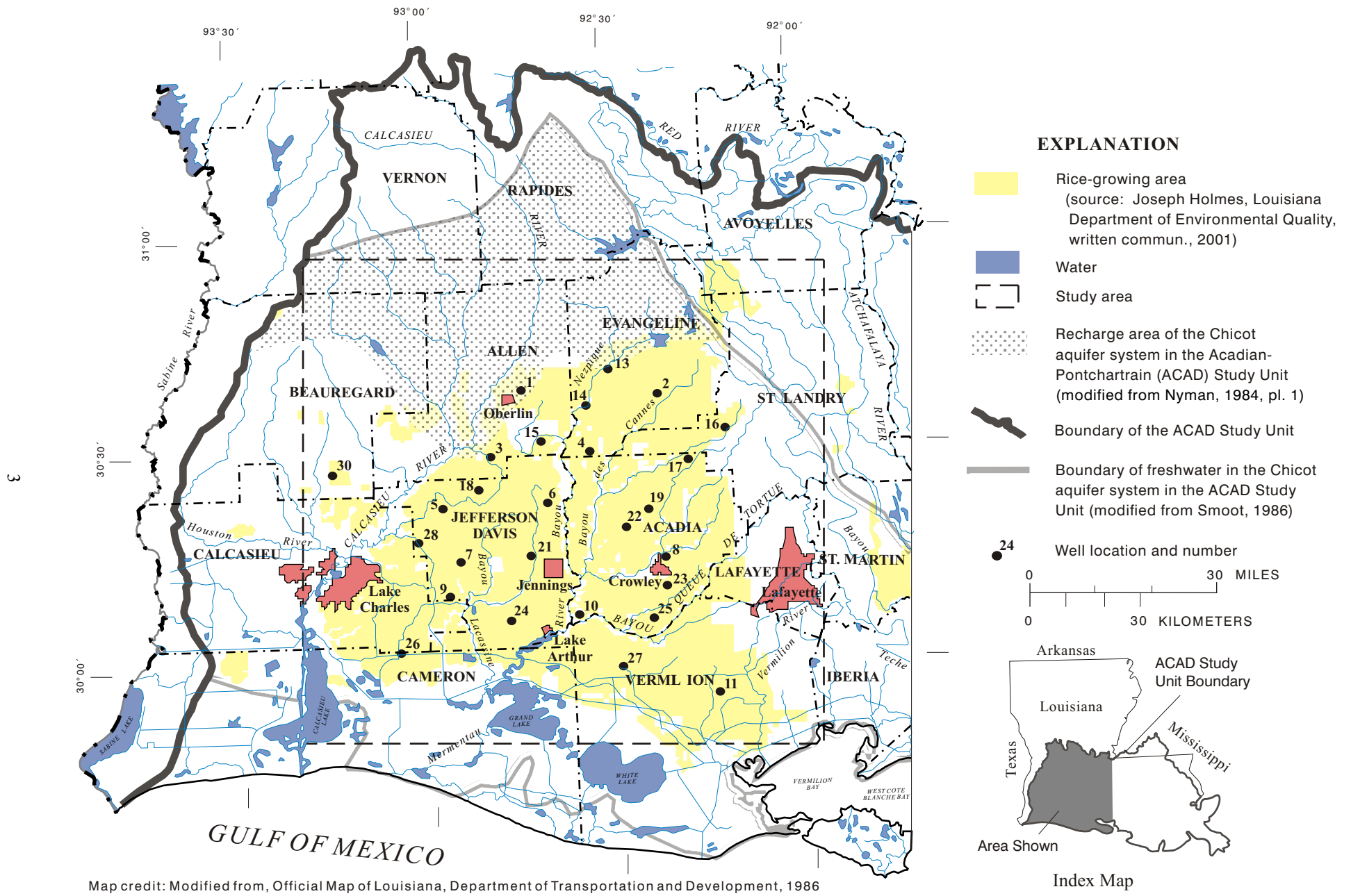
Figure 1. Study area and well locations in the rice-growing area in southwestern Louisiana in the Acadian-Pontchartrain Study Unit.
